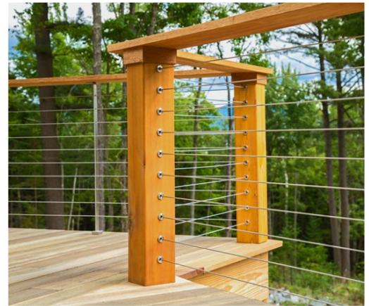
WOOD POST & CABLE RAILING for clear views from decks
