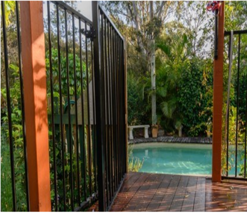
WOOD POST & ALUMINUM in pool code, flat top and bottom
